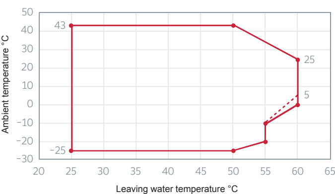
Heating mode
