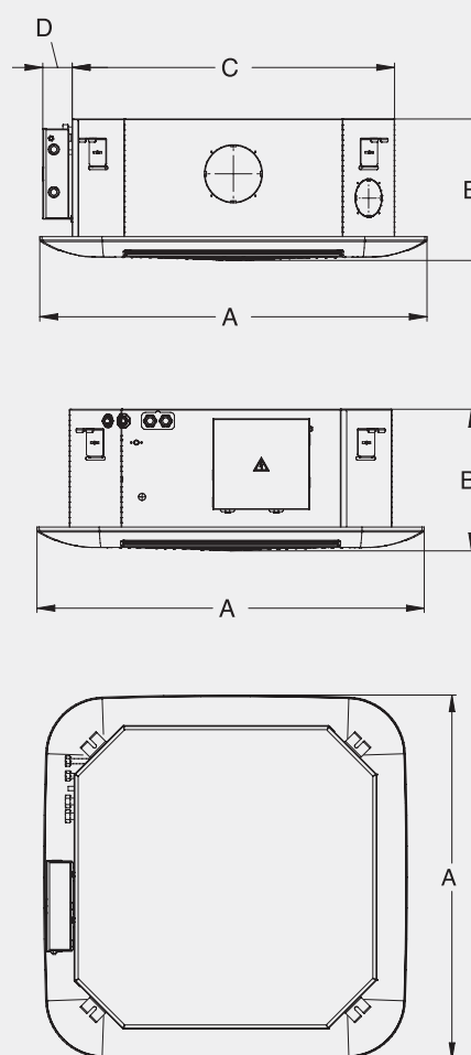
YKEY900 and YKEY900-ECM
