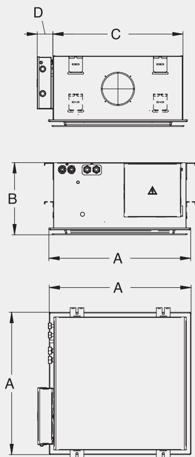
YKEY600 and YKEY600-ECM
