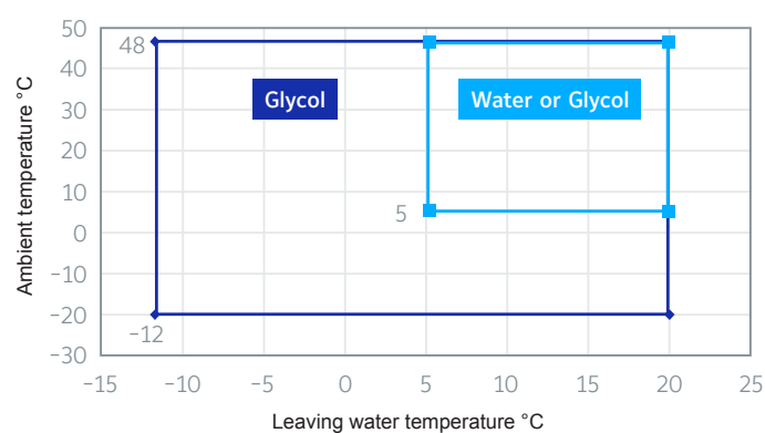
Cooling mode
