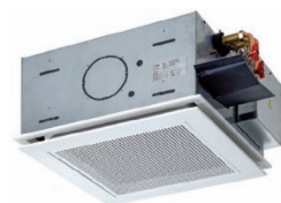
YKEY/M Special version with micro-drilled metallic grill
